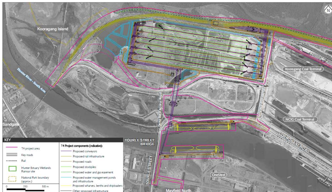
Figure 14 - PWCS Terminal 4 configuration as per Environmental Assessment
