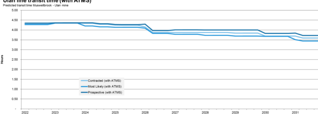
Figure 4-8 - Forecast transit time Muswellbrook - Ulan mine under contracted, most likely and prospective volume scenarios and works as per Table 4-1 with ATMS
