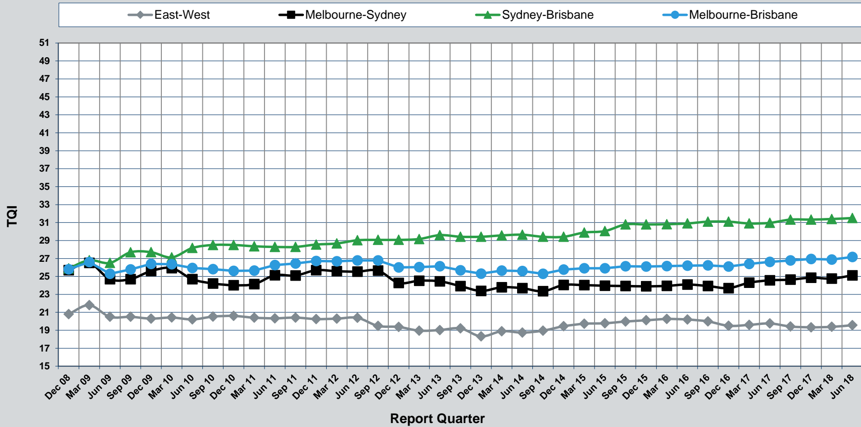
Track Quality Measured By Index (TQI)
