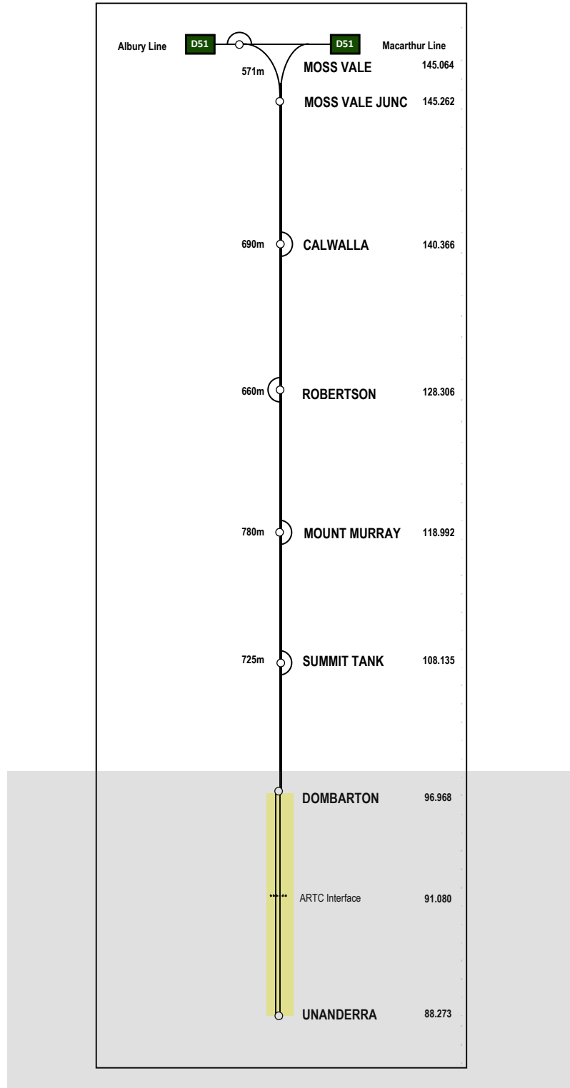
Track diagram updated to show dual track and Bi Directional operation.
