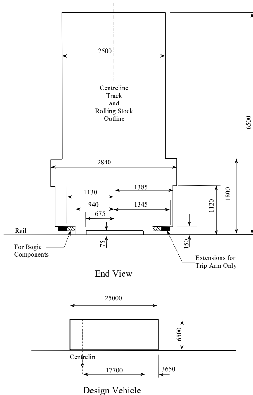
Figure A1.7 – Rolling Stock Interstate Outline Plate F2
