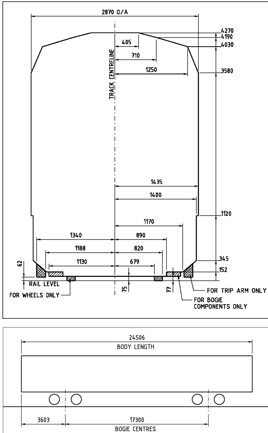
Figure A1.12 – Rolling Stock Outline Plate NSW Narrow Container (NC)
