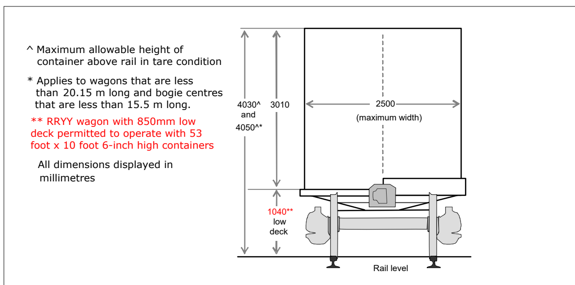
Figure A2.4 - Maximum Container Loading to meet Plates B, D, NC and IS
