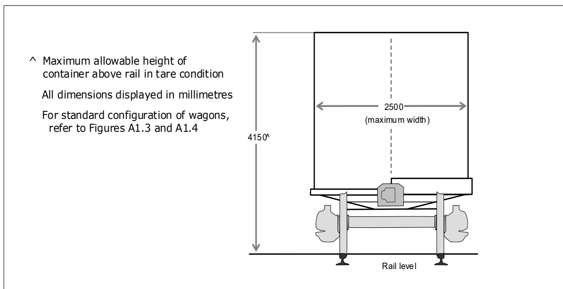
Figure A2.9.1 – Diagram for Area of Operation for Figure A2.9
